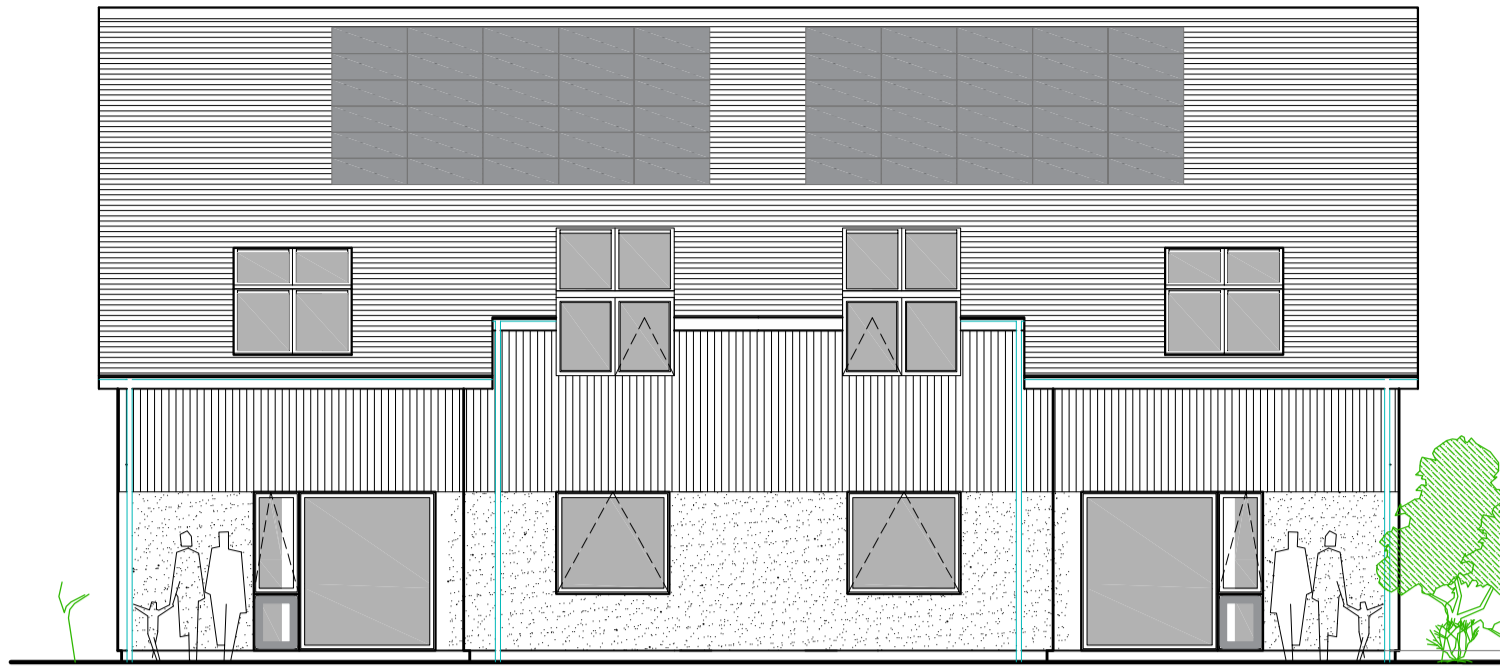
EDRYCHIAD CEFN REAR ELEVATION
